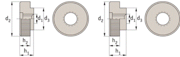
Type 1 - Short Collar
